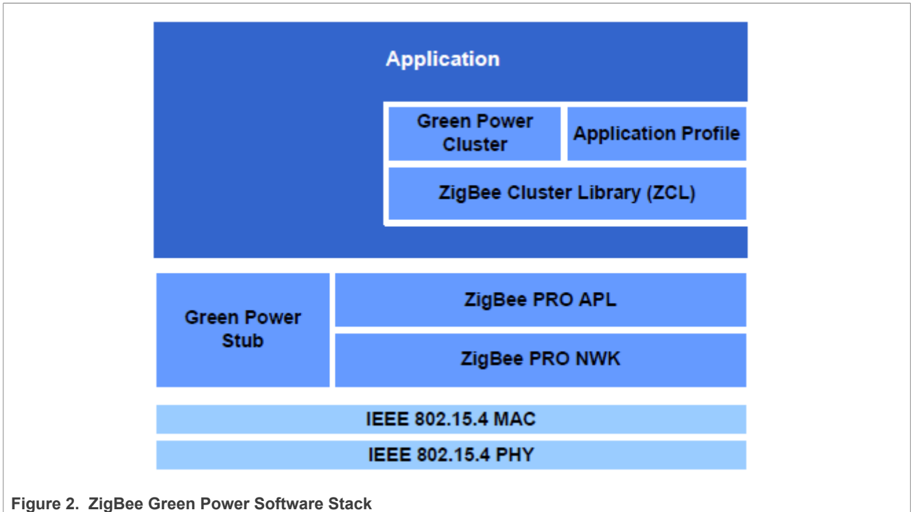
Figure 2. ZigBee Green Power Software Stack
