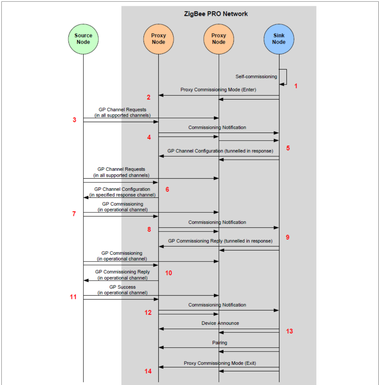
Figure 6. Example of green power bi-directional commissioning mode
