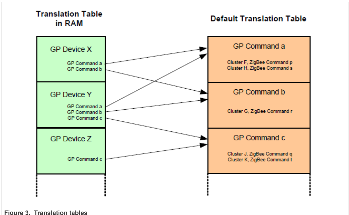
Figure 3. Translation tables
