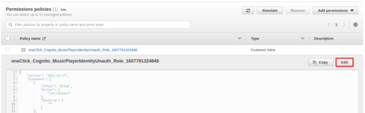
Figure 69: Edit the policy
